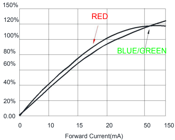
Typical Relative Luminous Flux vs. Forward Current
