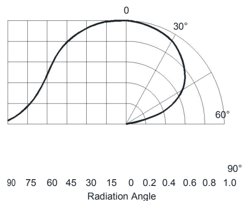
Typical Radiation Pattern 120°
